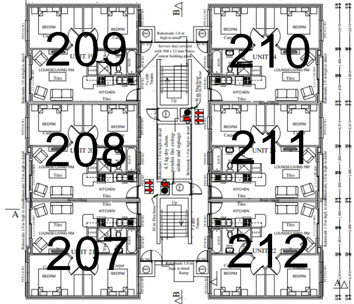
FIRST FLOOR LAYOUT PLAN
